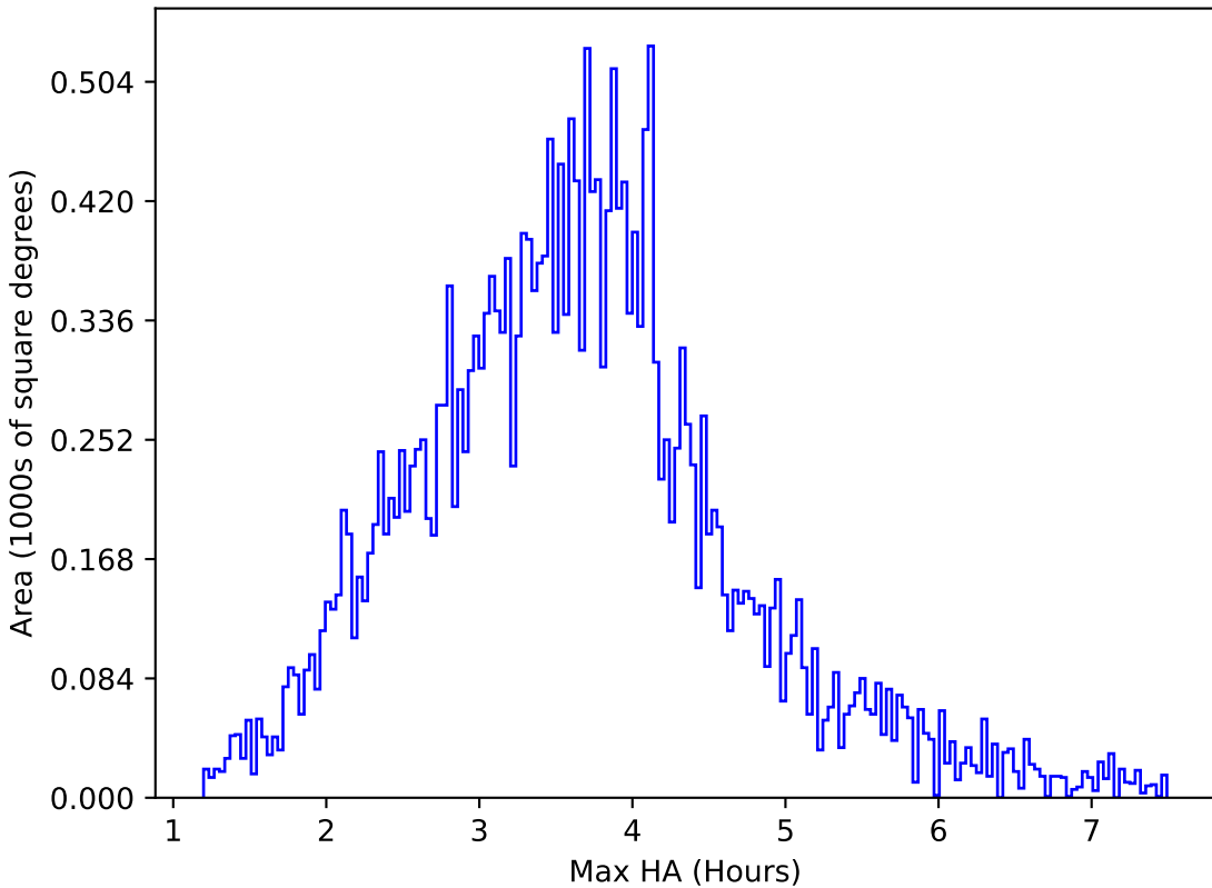
start_date_do90v3.4_10yrs All sky g band: Max HA
