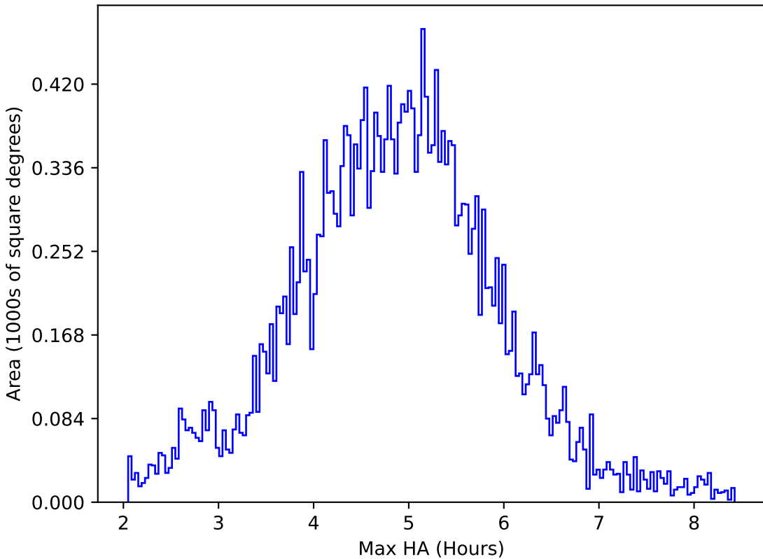
start_date_do90v3.4_10yrs All sky all bands: Max HA
