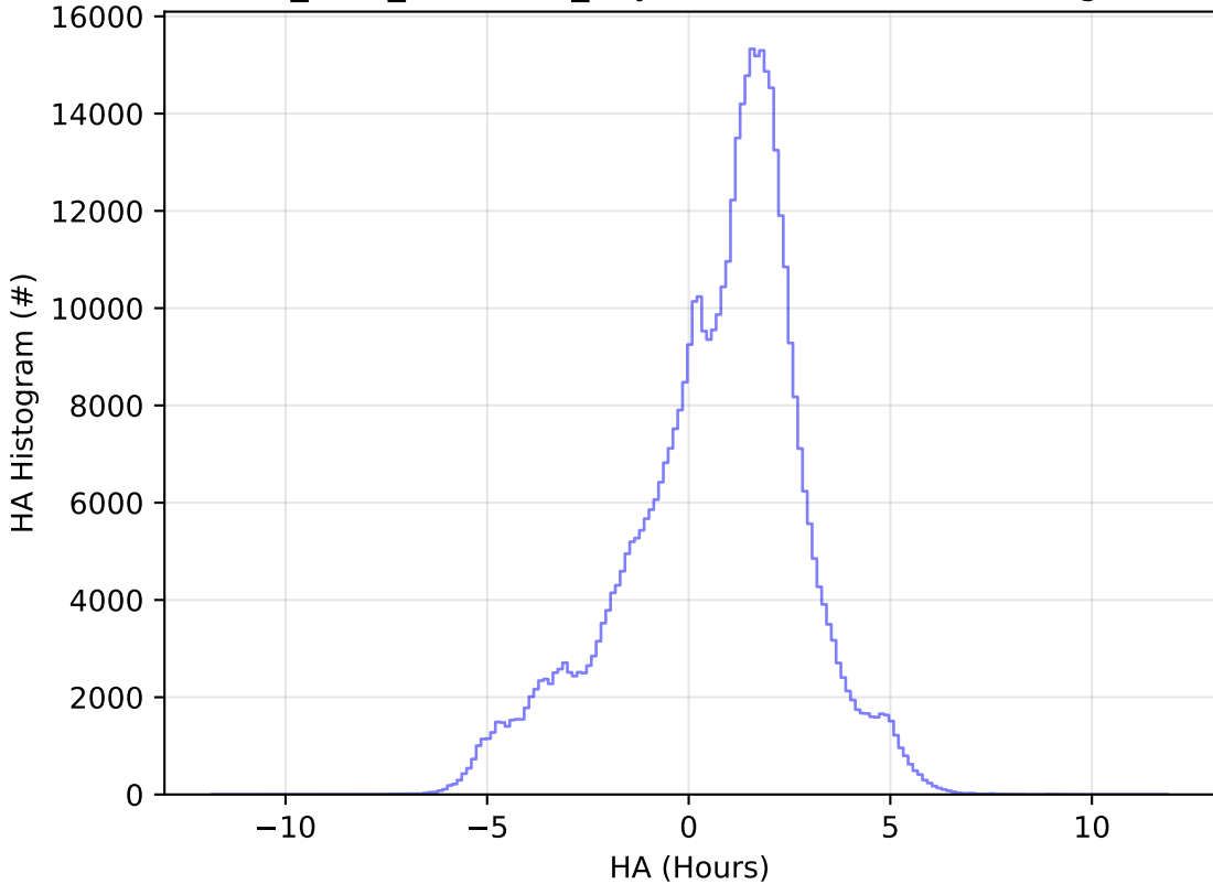
start_date_do90v3.4_10yrs WFD i band: HA Histogram
