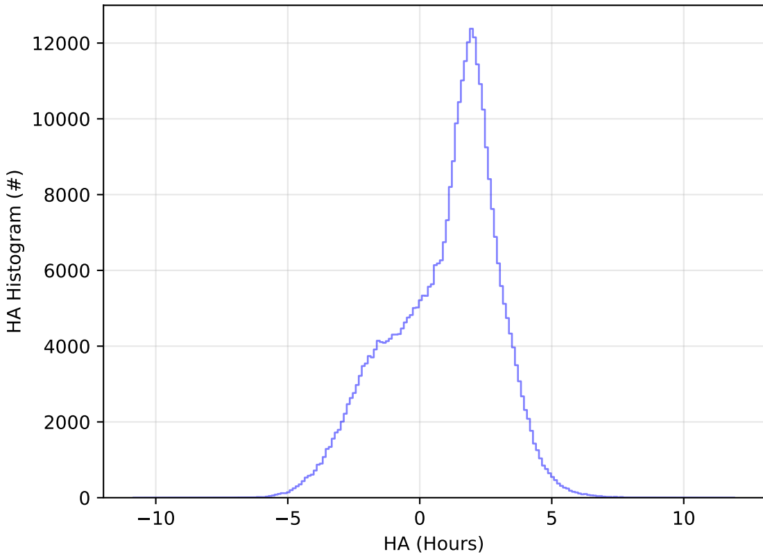
start_date_do90v3.4_10yrs All sky y band: HA Histogram
