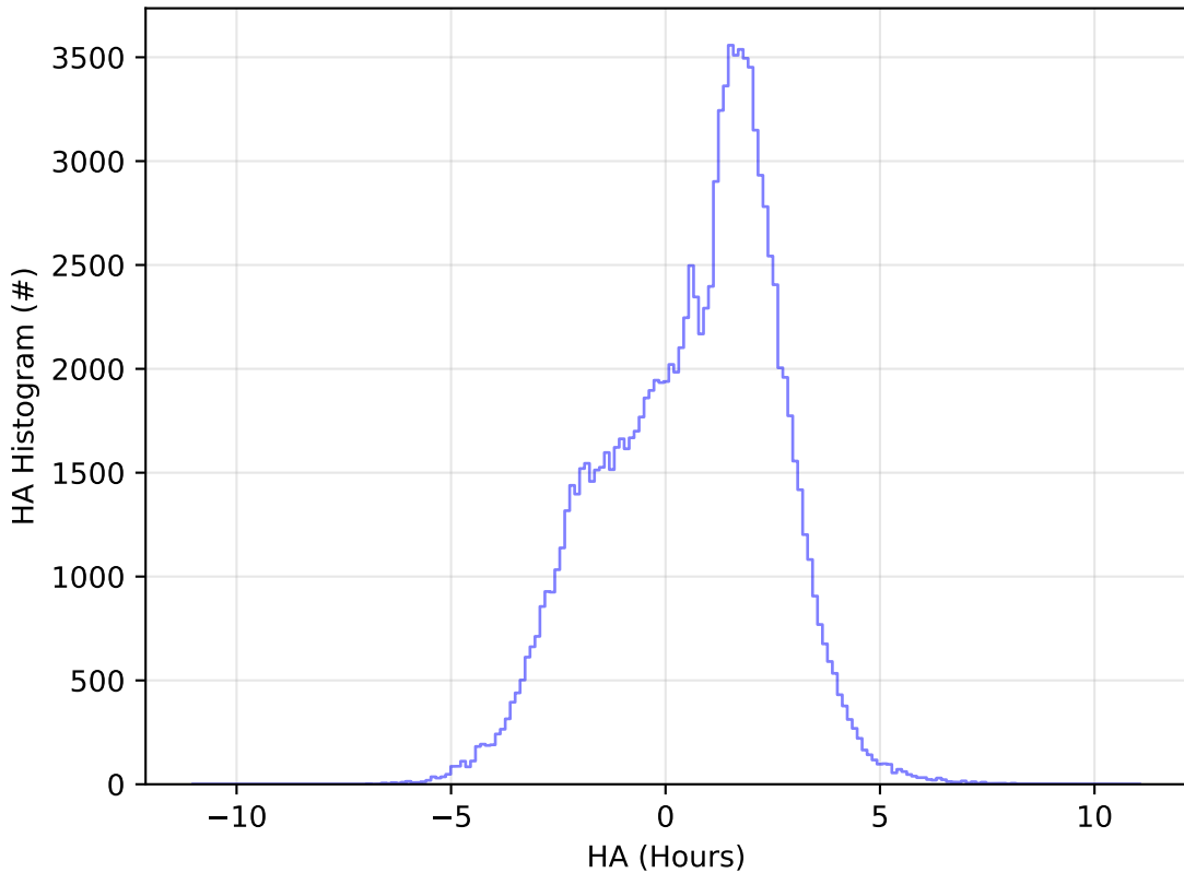
start_date_do90v3.4_10yrs All sky u band: HA Histogram
