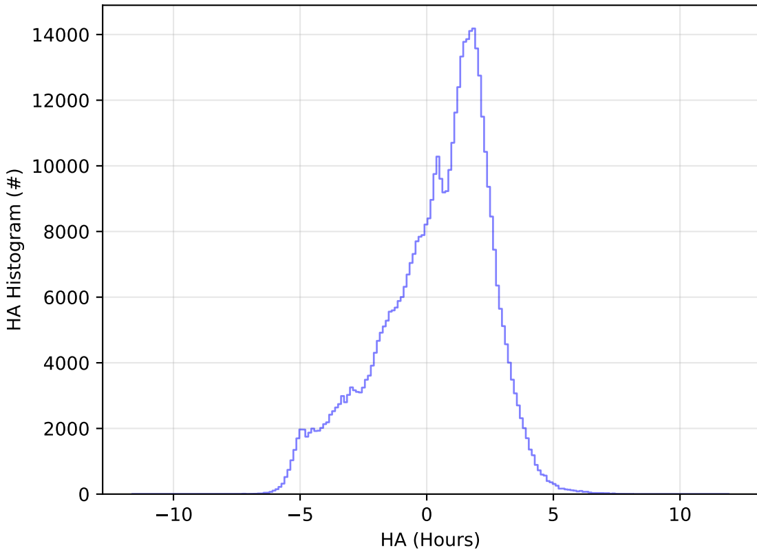
start_date_do90v3.4_10yrs All sky r band: HA Histogram
