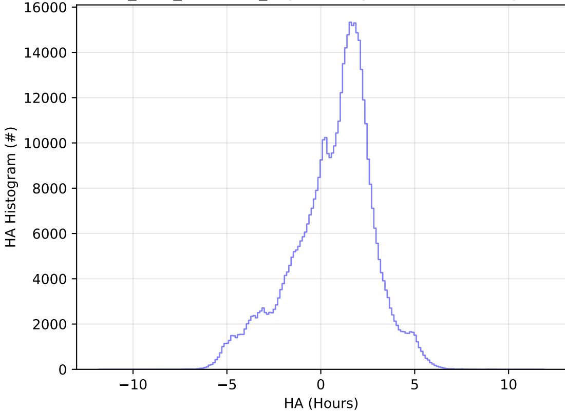
start_date_do90v3.4_10yrs All sky i band: HA Histogram
