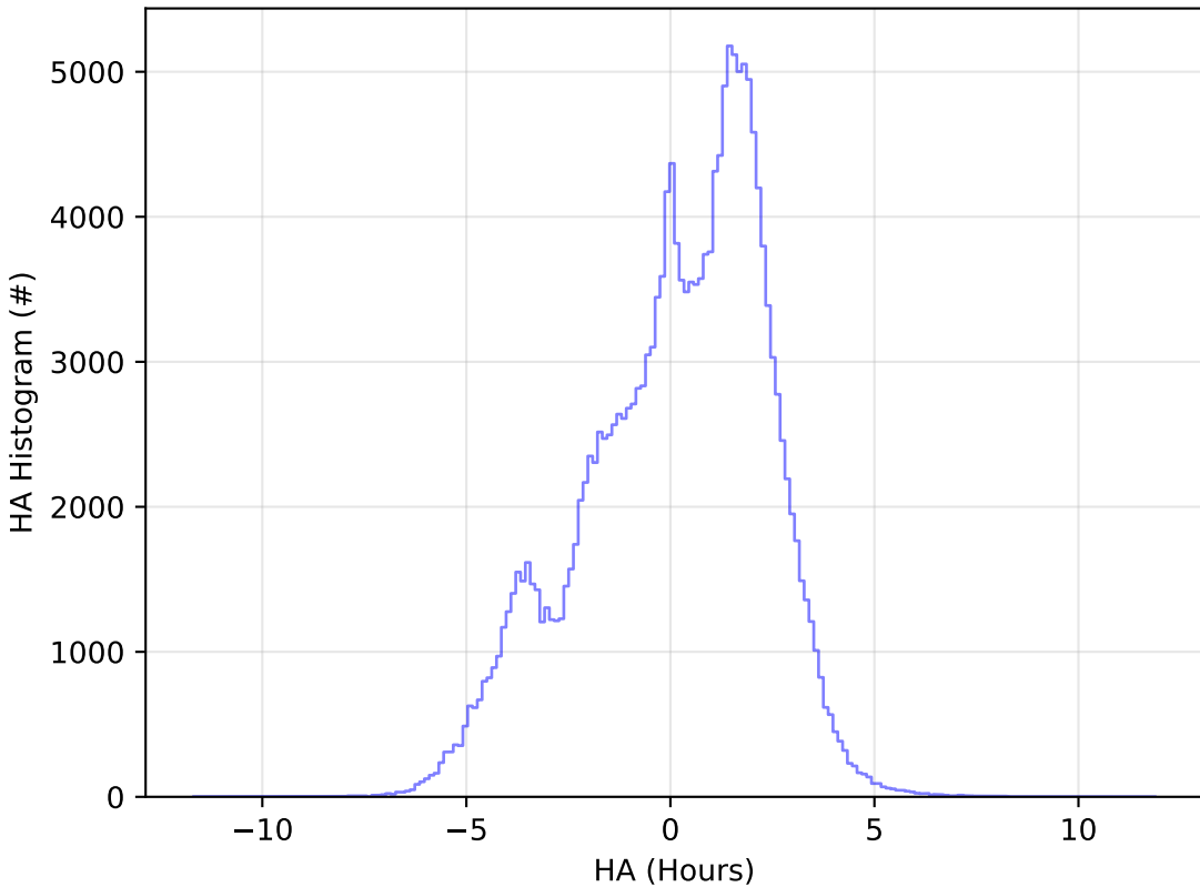
start_date_do90v3.4_10yrs All sky g band: HA Histogram
