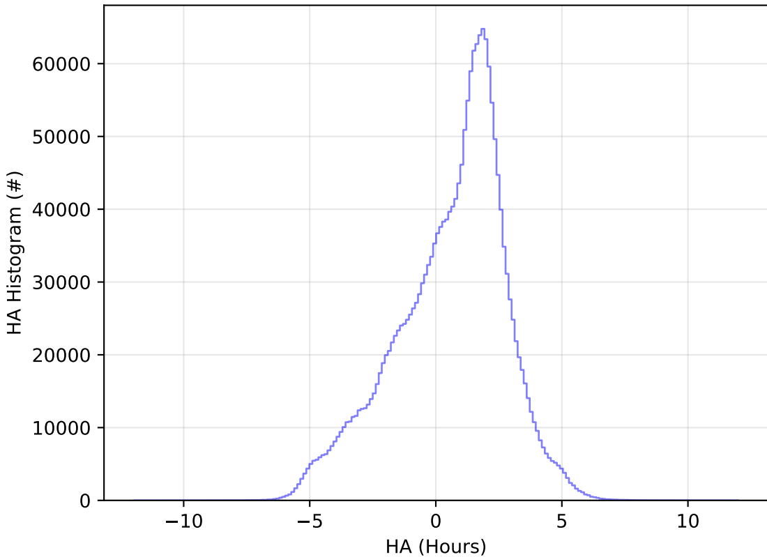
start_date_do90v3.4_10yrs All sky all bands: HA Histogram
