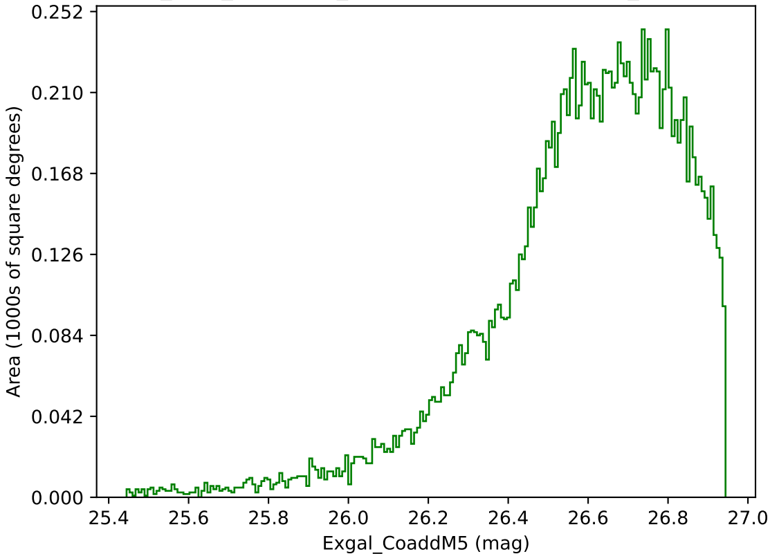
start_date_do90v3.4_10yrs WFD g band: Exgal_CoaddM5
