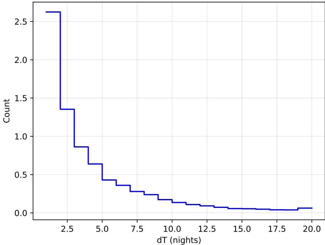
start_date_do90v3.4_10yrs WFD all bands: DeltaNight Histogram 1e6
