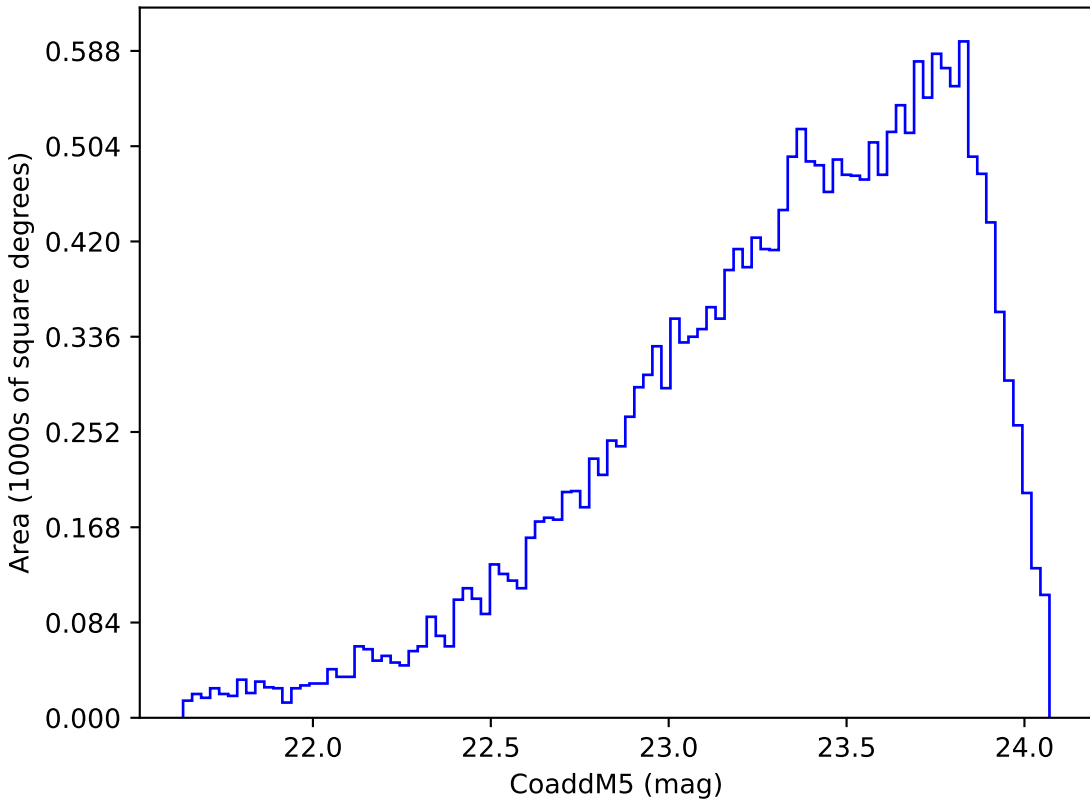
start_date_do90v3.4_10yrs Yr 3-4 y band: CoaddM5
