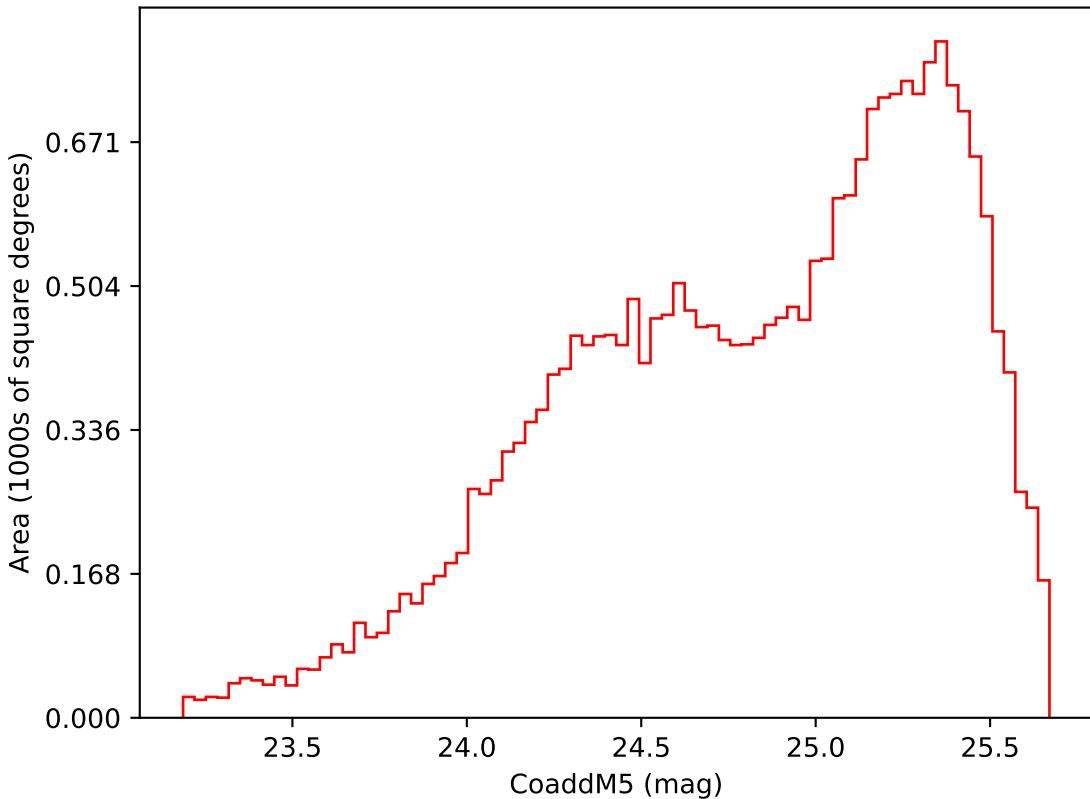
start_date_do90v3.4_10yrs Yr 3-4 i band: CoaddM5
