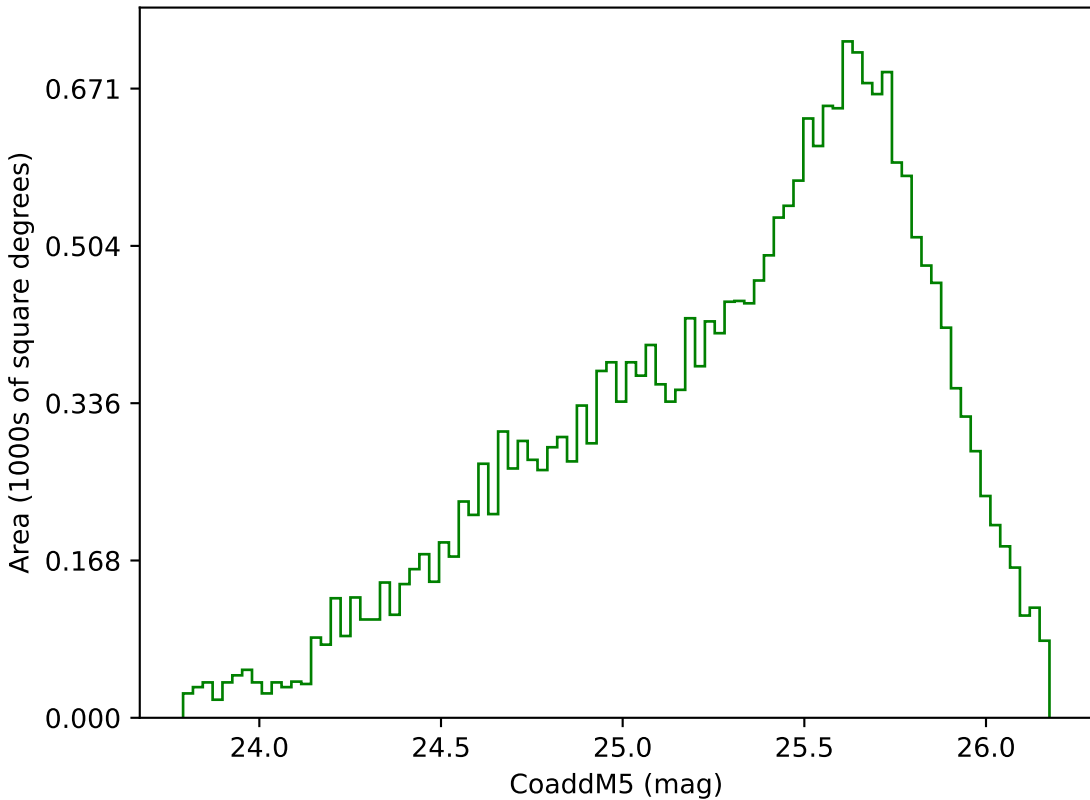
start_date_do90v3.4_10yrs Yr 3-4 g band: CoaddM5
