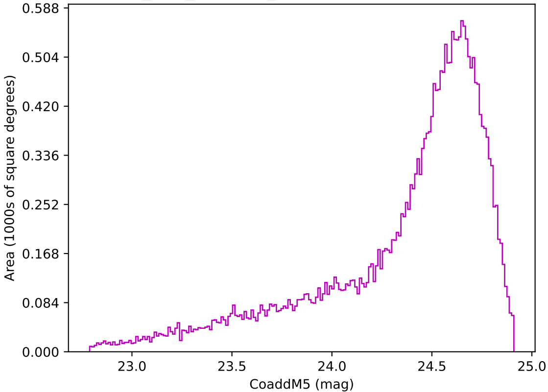
start_date_do90v3.4_10yrs Yr 1 z band: CoaddM5
