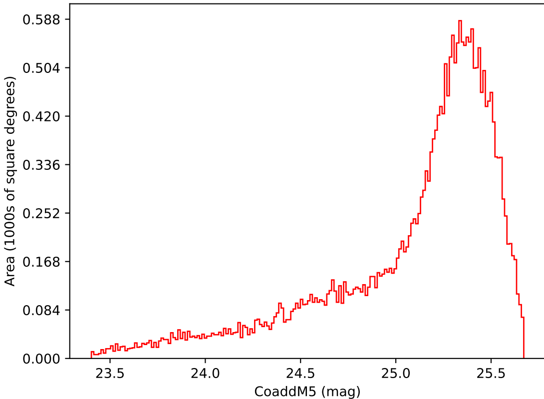
start_date_do90v3.4_10yrs Yr 1 i band: CoaddM5
