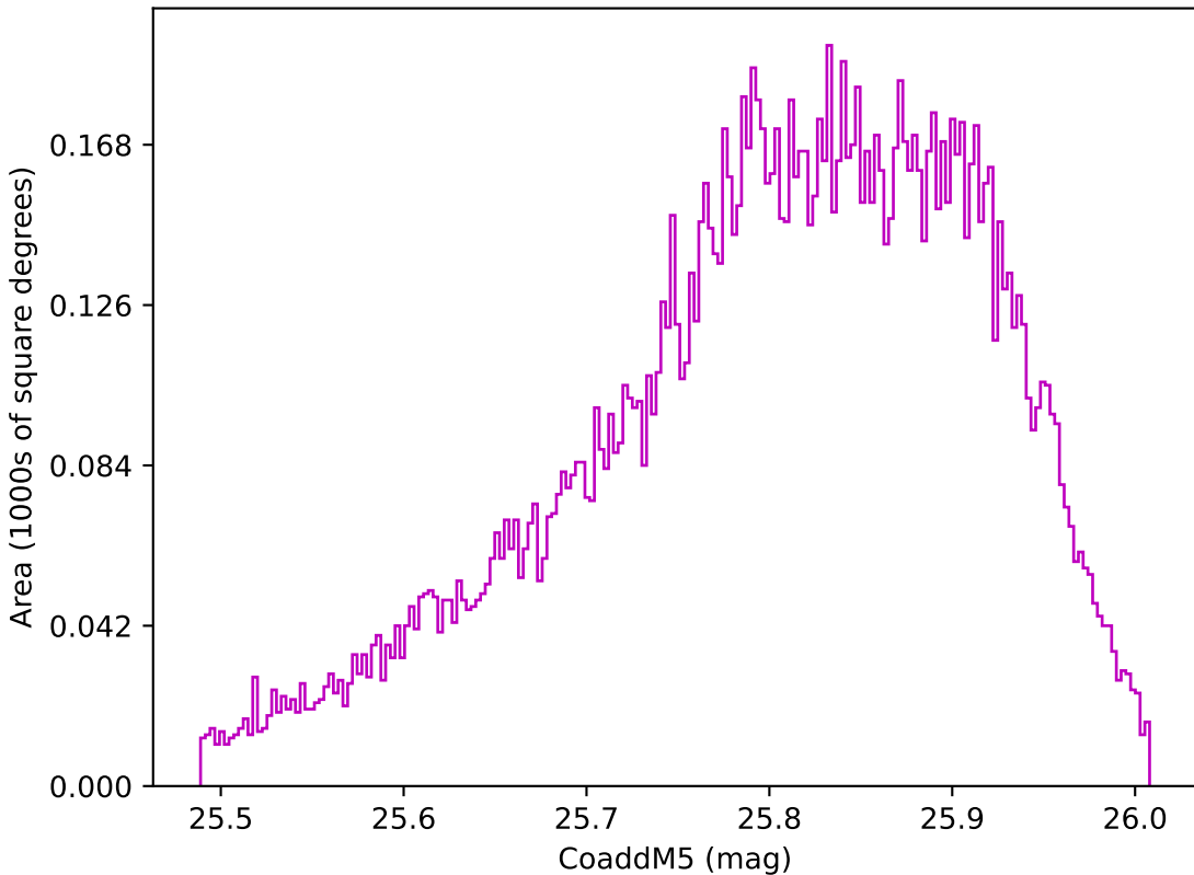
start_date_do90v3.4_10yrs WFD z band: CoaddM5
