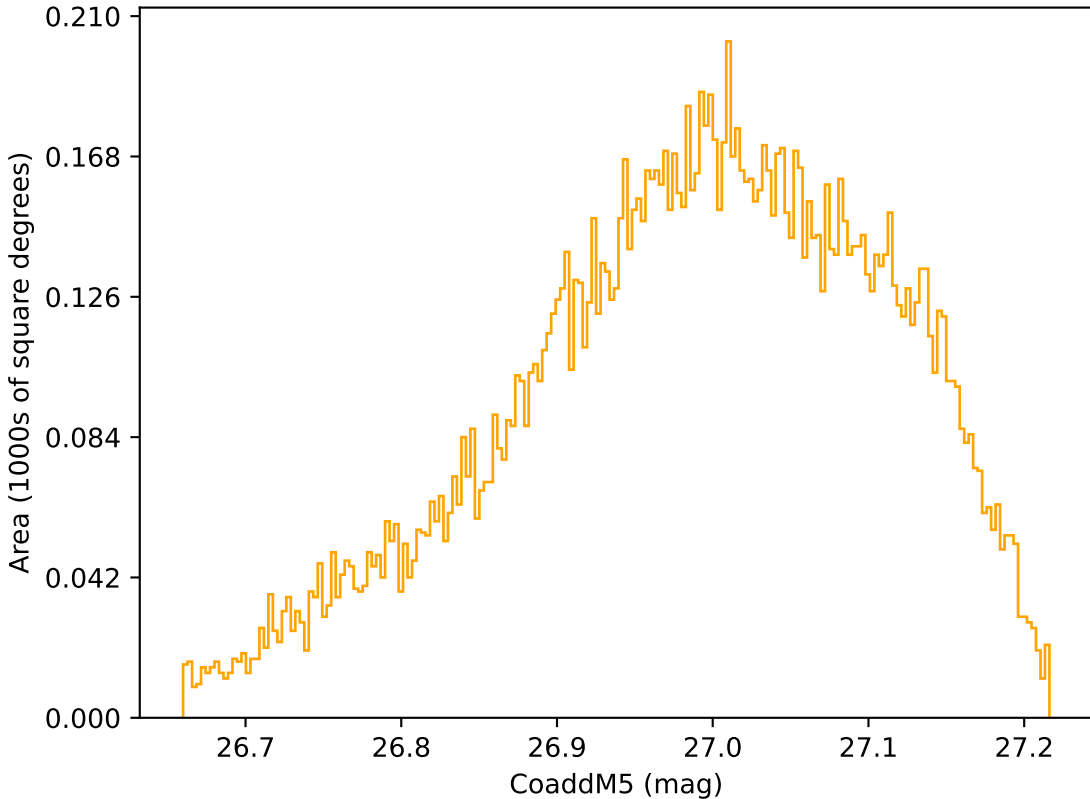
start_date_do90v3.4_10yrs WFD r band: CoaddM5
