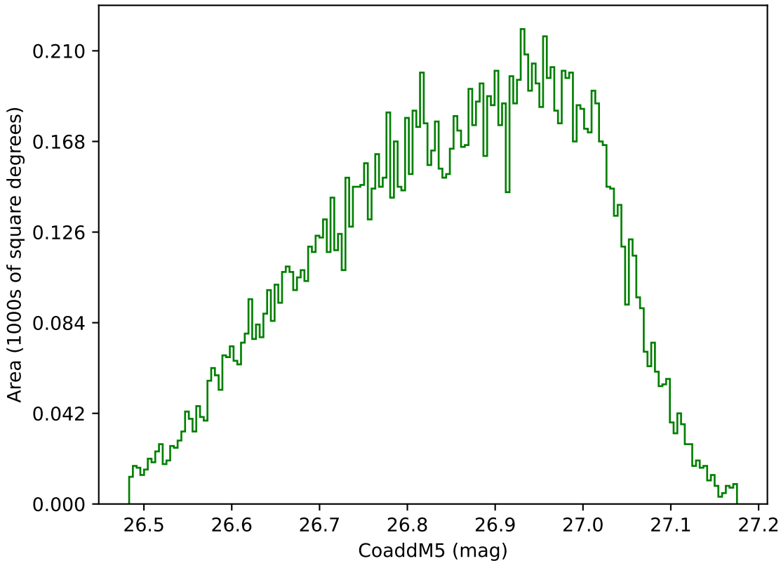
start_date_do90v3.4_10yrs WFD g band: CoaddM5
