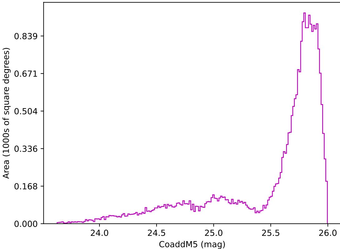
start_date_do90v3.4_10yrs All sky z band: CoaddM5
