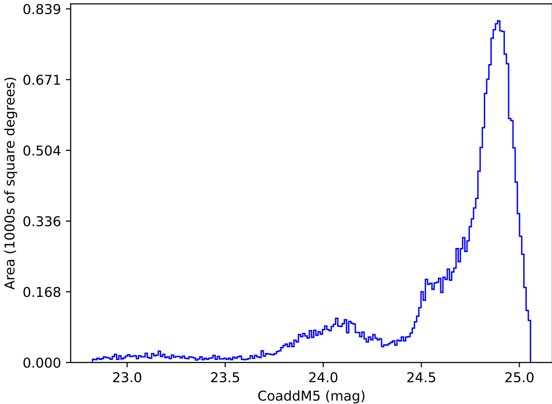
start_date_do90v3.4_10yrs All sky y band: CoaddM5
