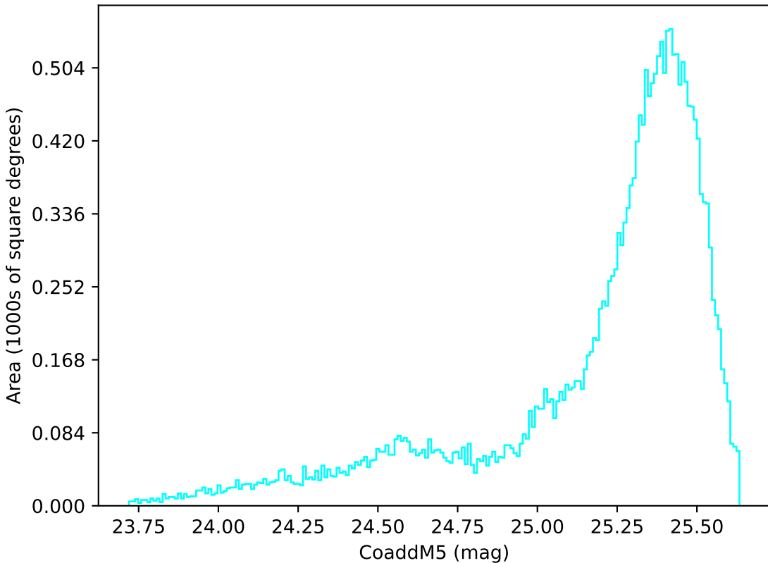
start_date_do90v3.4_10yrs All sky u band: CoaddM5
