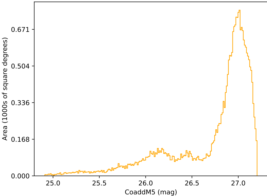
start_date_do90v3.4_10yrs All sky r band: CoaddM5
