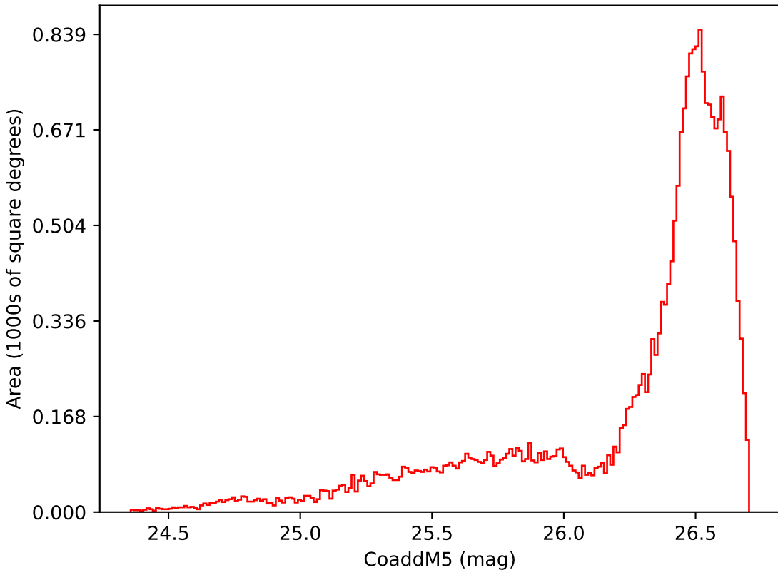
start_date_do90v3.4_10yrs All sky i band: CoaddM5
