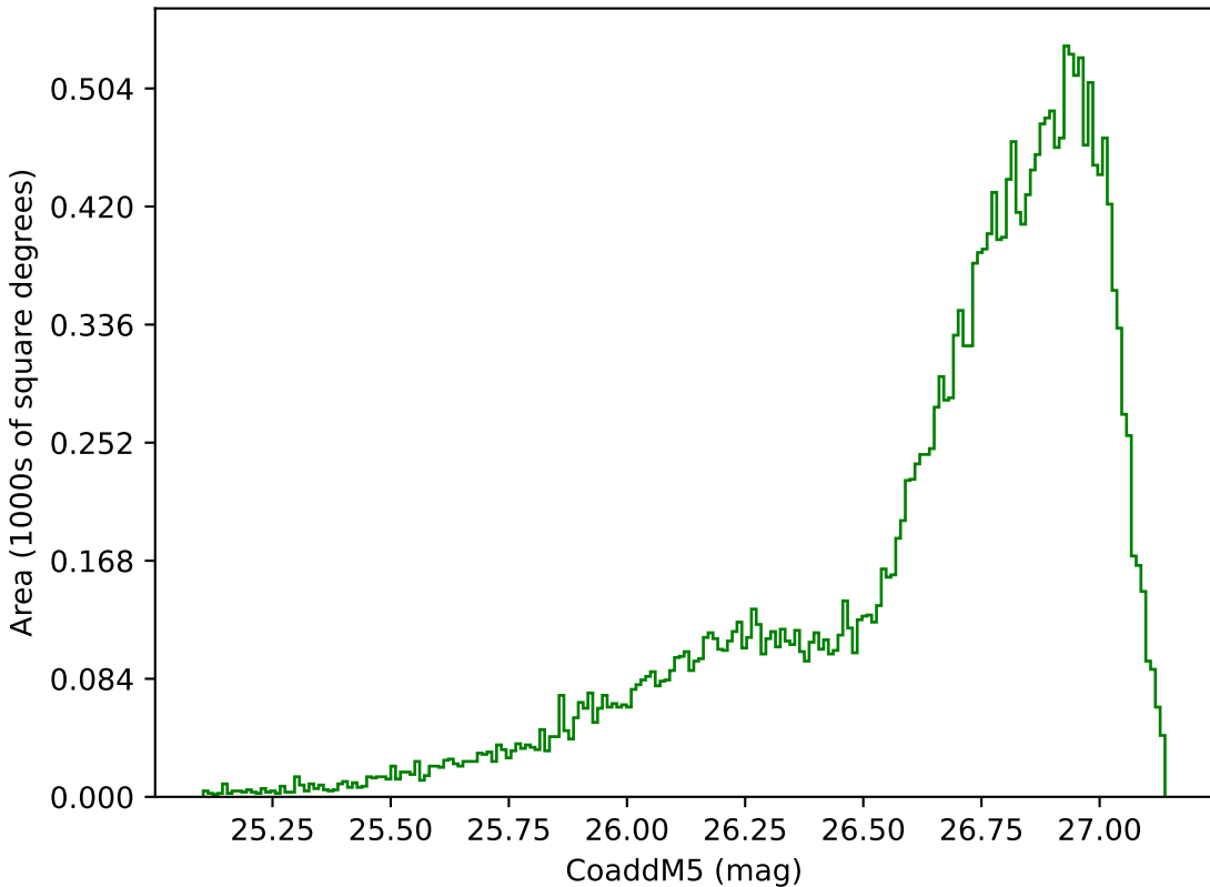
start_date_do90v3.4_10yrs All sky g band: CoaddM5
