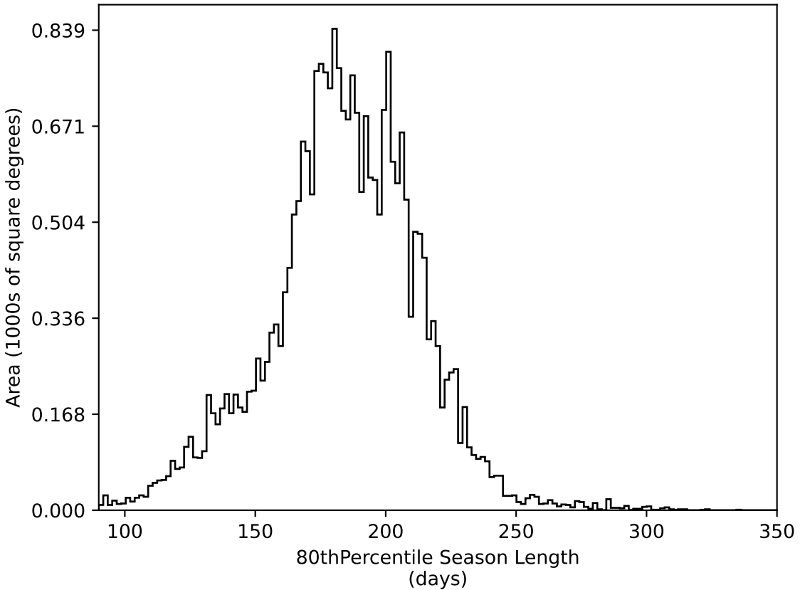
start_date_do90v3.4_10yrs All sky all bands: 80thPercentile Season Length
