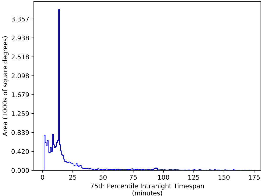
start_date_do90v3.4_10yrs WFD z band: 75th Percentile Intranight Timespan
