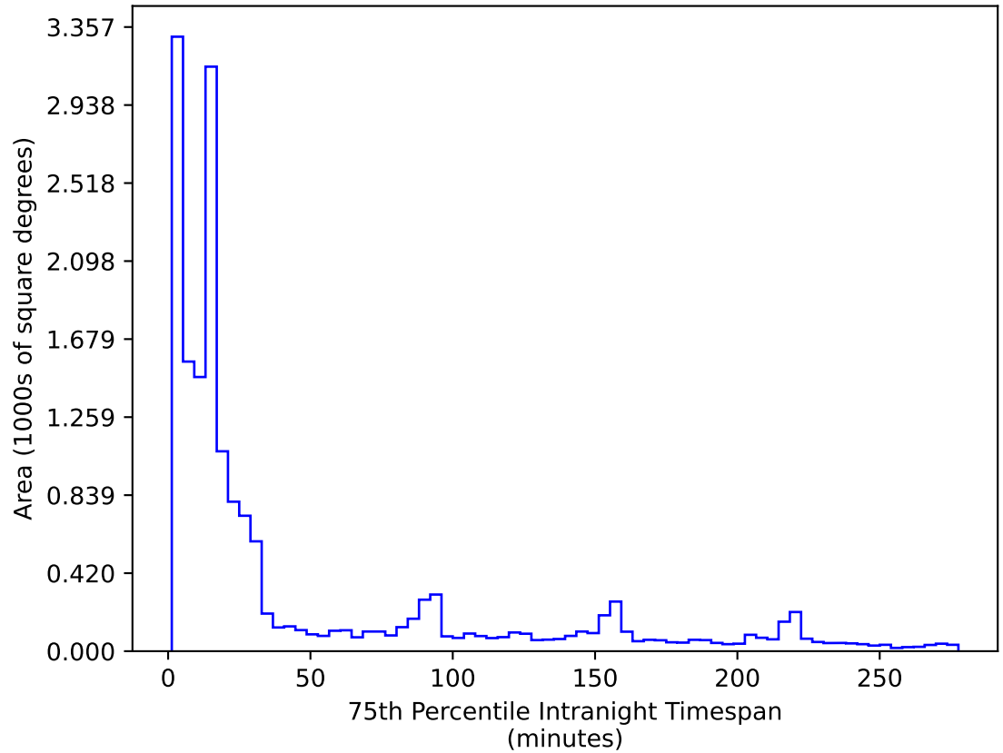
start_date_do90v3.4_10yrs WFD r band: 75th Percentile Intranight Timespan
