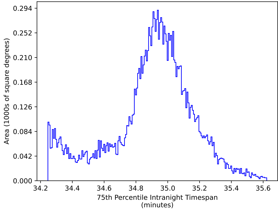
start_date_do90v3.4_10yrs WFD all bands: 75th Percentile Intranight Timespan
