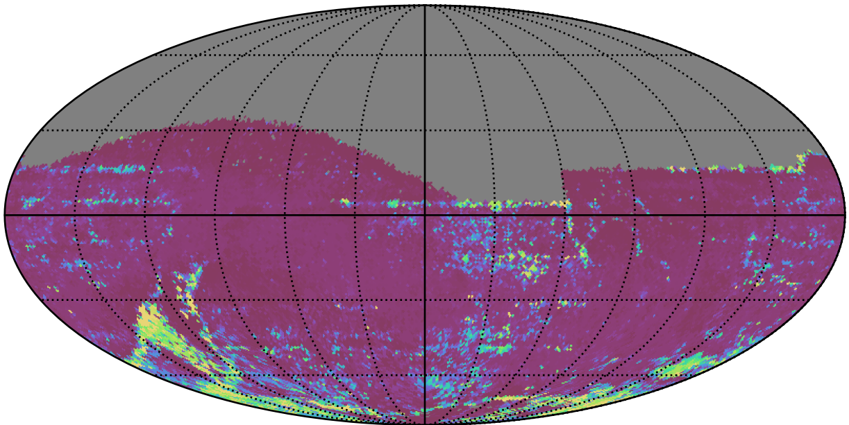
start_date_do90v3.4_10yrs All sky z band: 75th Percentile Intranight Timespan
