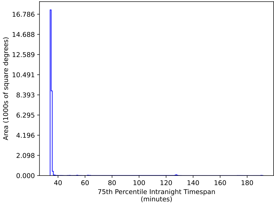
start_date_do90v3.4_10yrs All sky iz bands: 75th Percentile Intranight Timespan
