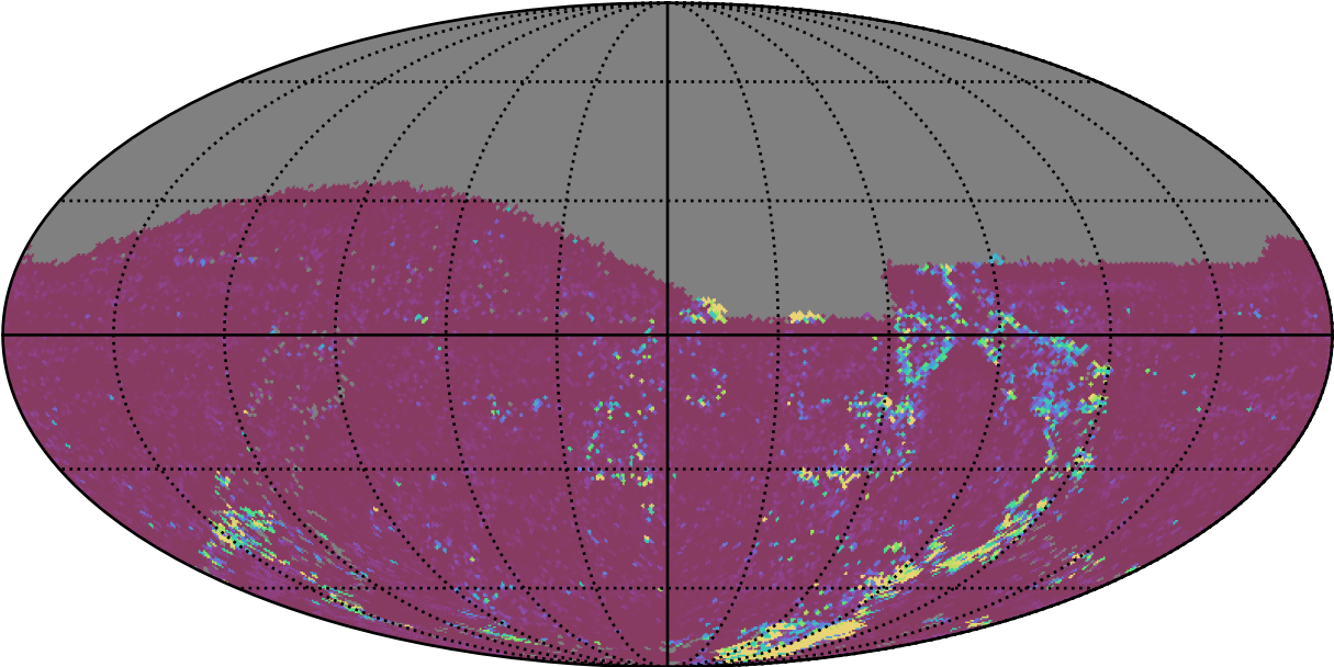
start_date_do90v3.4_10yrs All sky g band: 75th Percentile Intranight Timespan
