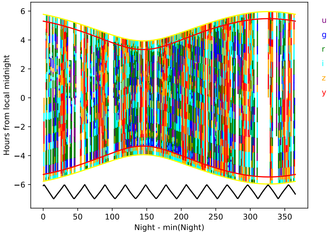
start_date_do90v3.4_10yrs year 9-10: Hourglass
