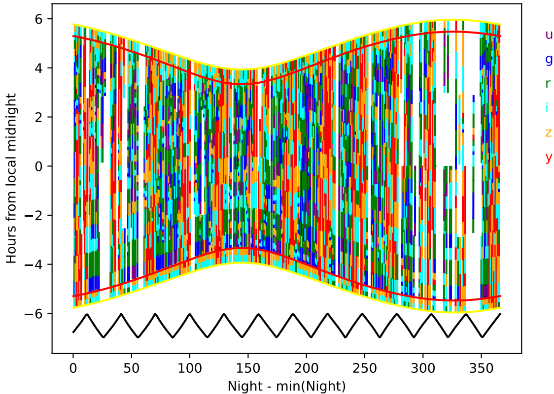
start_date_do90v3.4_10yrs year 8-9: Hourglass
