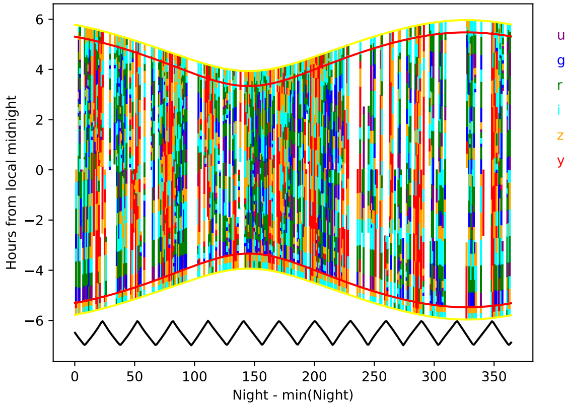
start_date_do90v3.4_10yrs year 7-8: Hourglass
