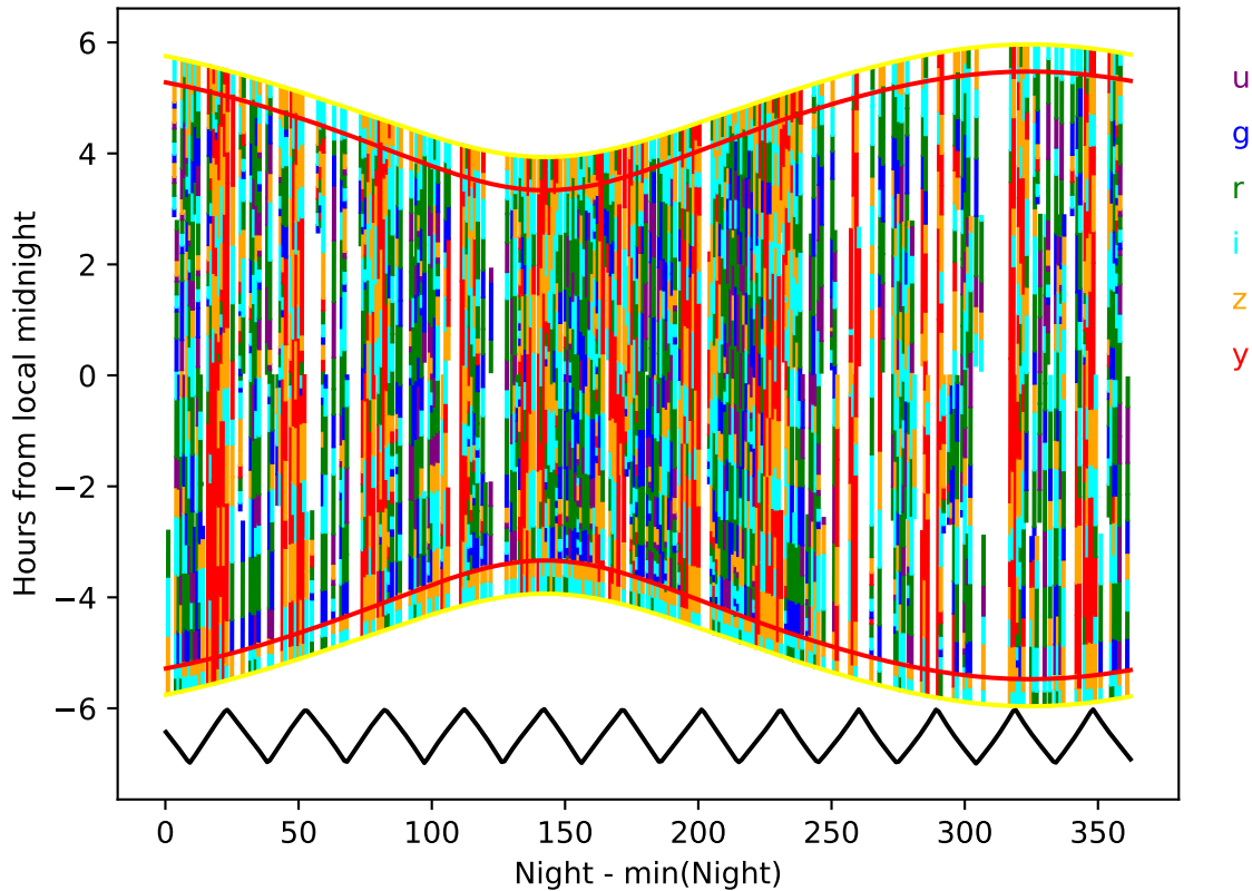
start_date_do90v3.4_10yrs year 4-5: Hourglass
