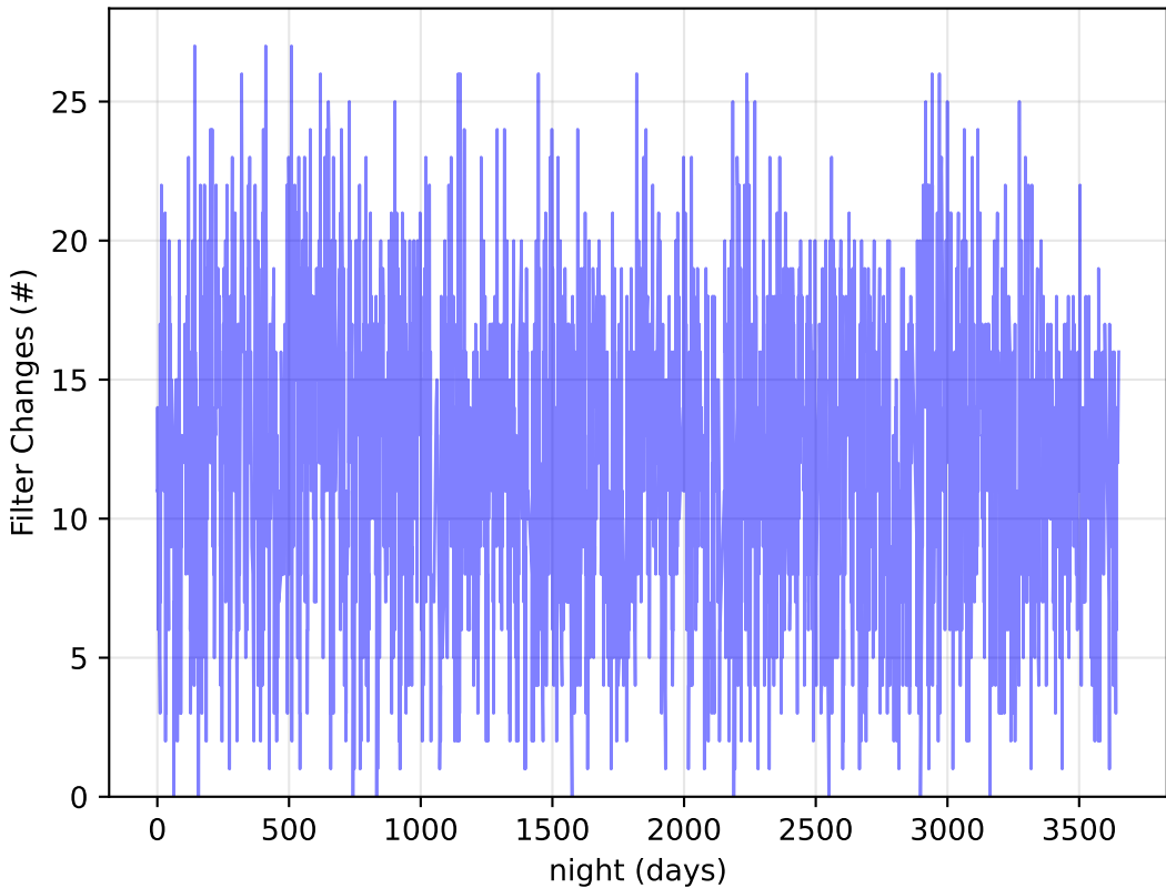
start_date_do90v3.4_10yrs : Filter Changes
