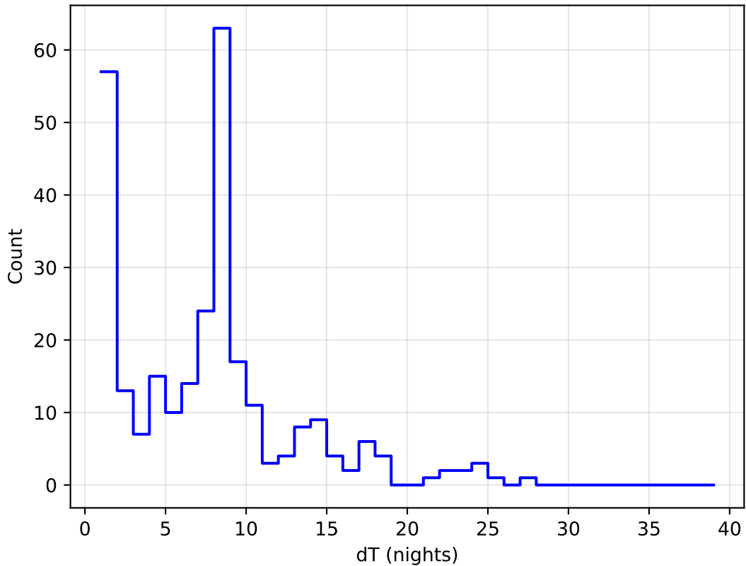
start_date_do90v3.4_10yrs all bands: DD:XMM_LSS Delta Nights Histogram
