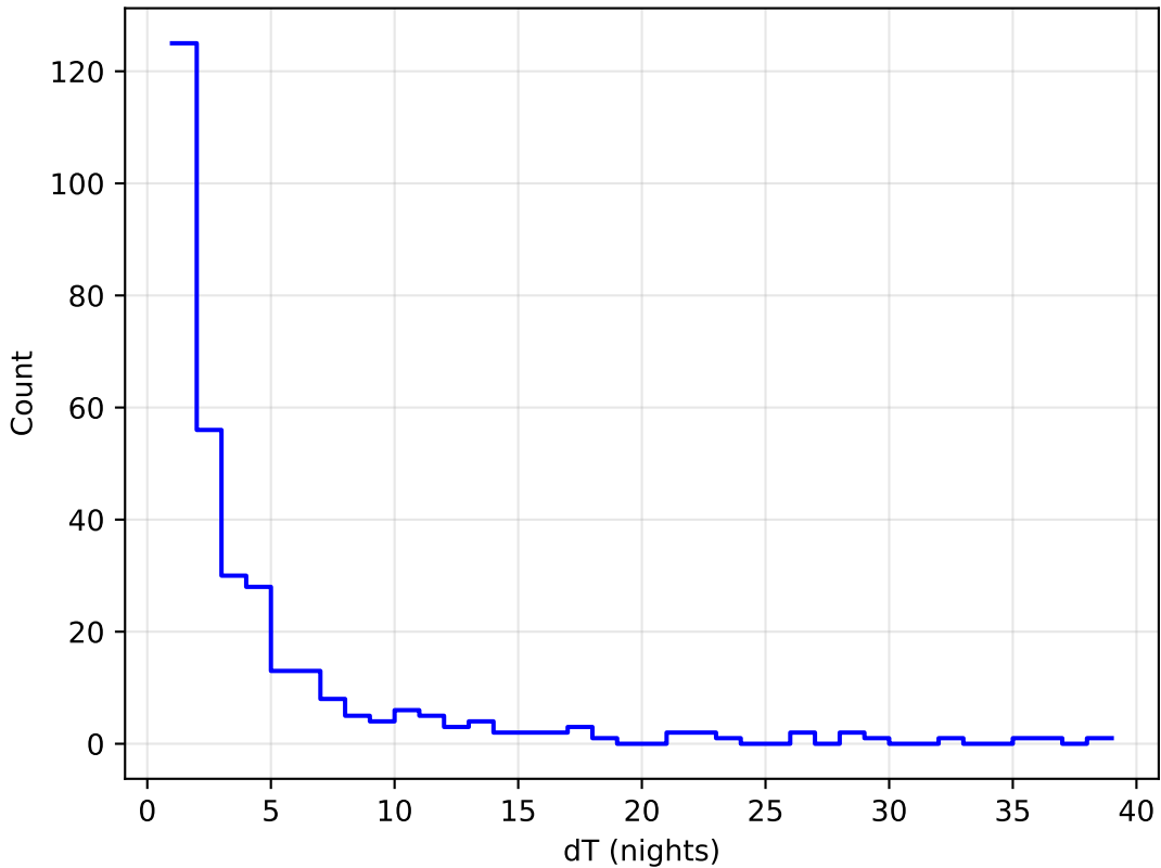
start_date_do90v3.4_10yrs all bands: DD:WFD Delta Nights Histogram
