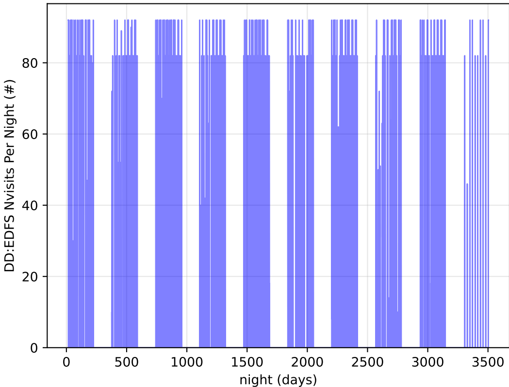
start_date_do90v3.4_10yrs all bands: DD:EDFS Nvisits Per Night
