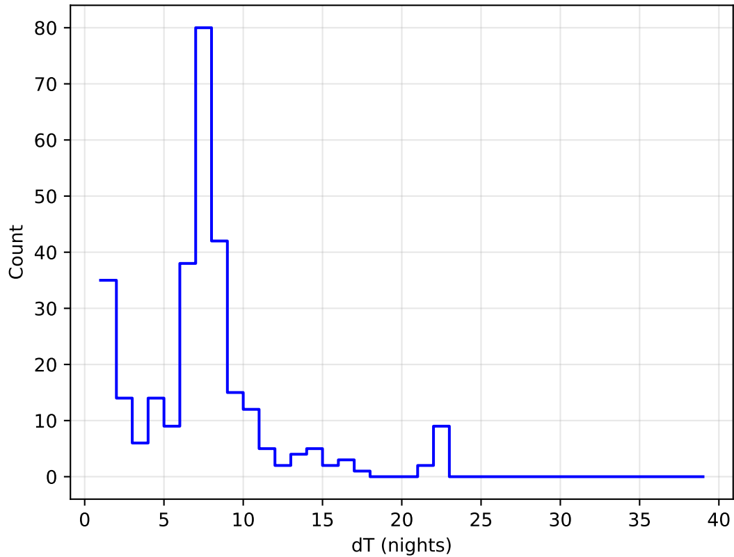
start_date_do90v3.4_10yrs all bands: DD:EDFS Delta Nights Histogram
