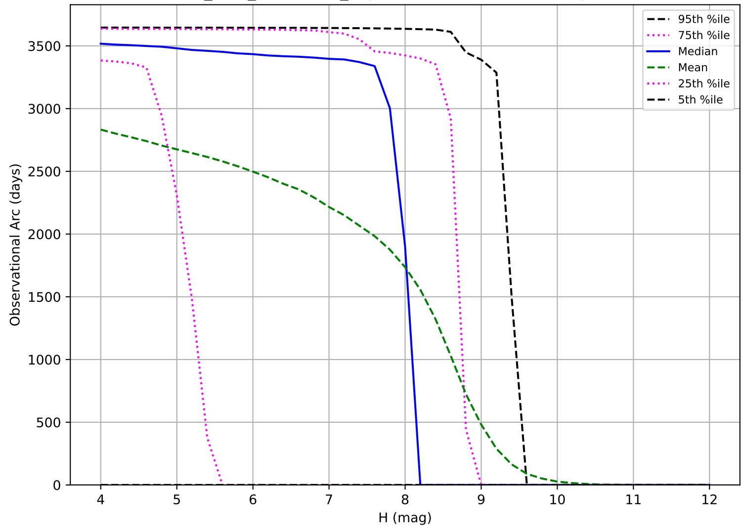
start_date_do360v3.4_10yrs: Observational Arc Length TNO
