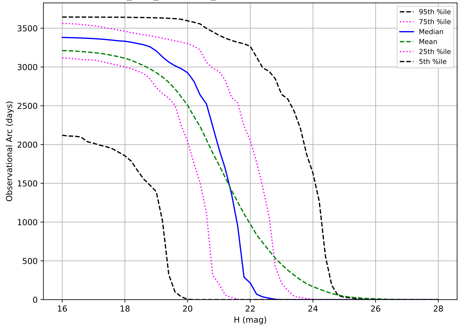
start_date_do360v3.4_10yrs: Observational Arc Length PHA
