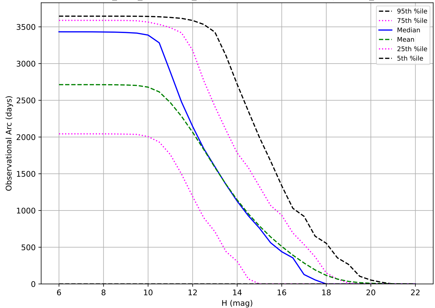
start_date_do360v3.4_10yrs: Observational Arc Length OCC_r5
