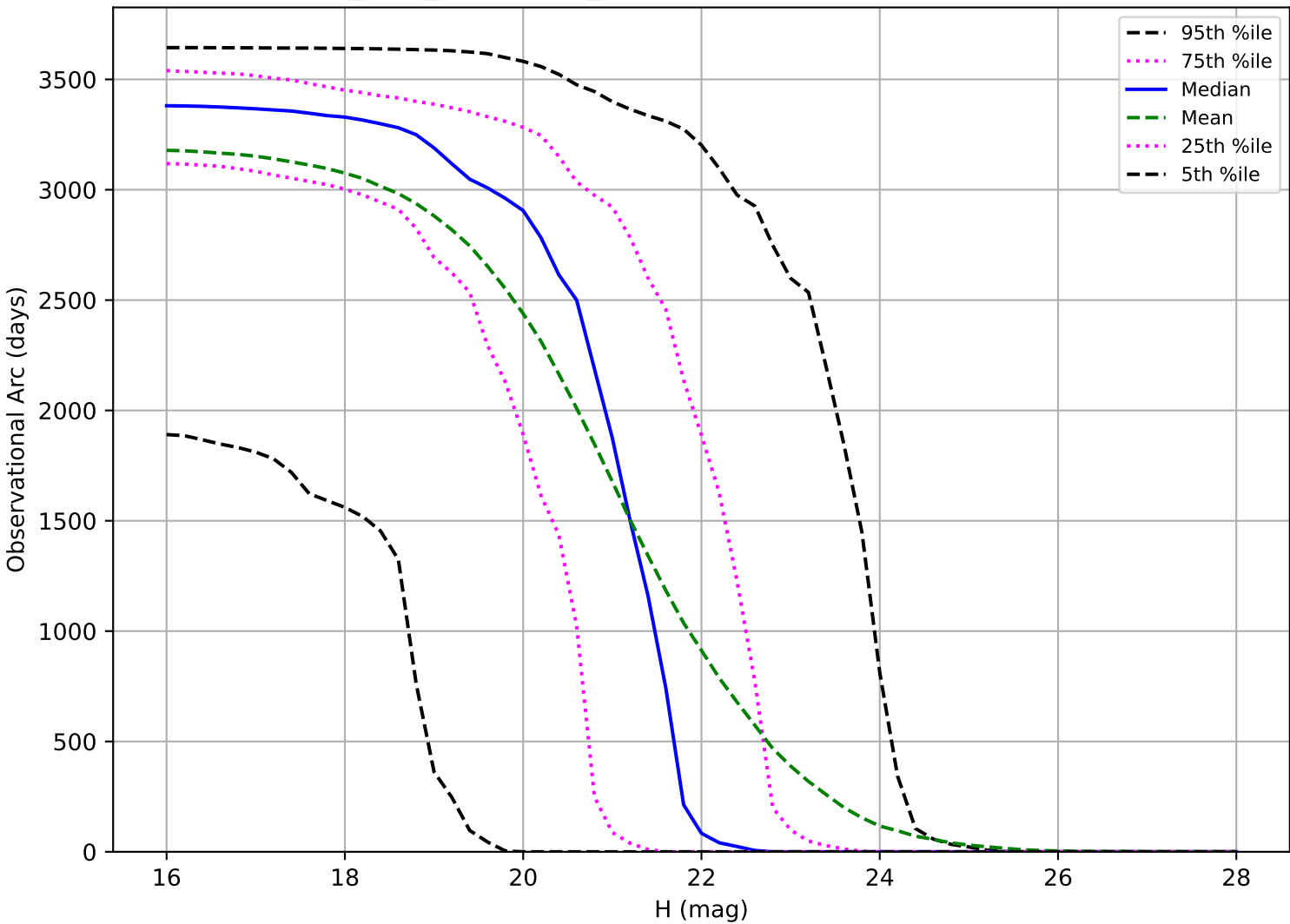
start_date_do360v3.4_10yrs: Observational Arc Length NEO
