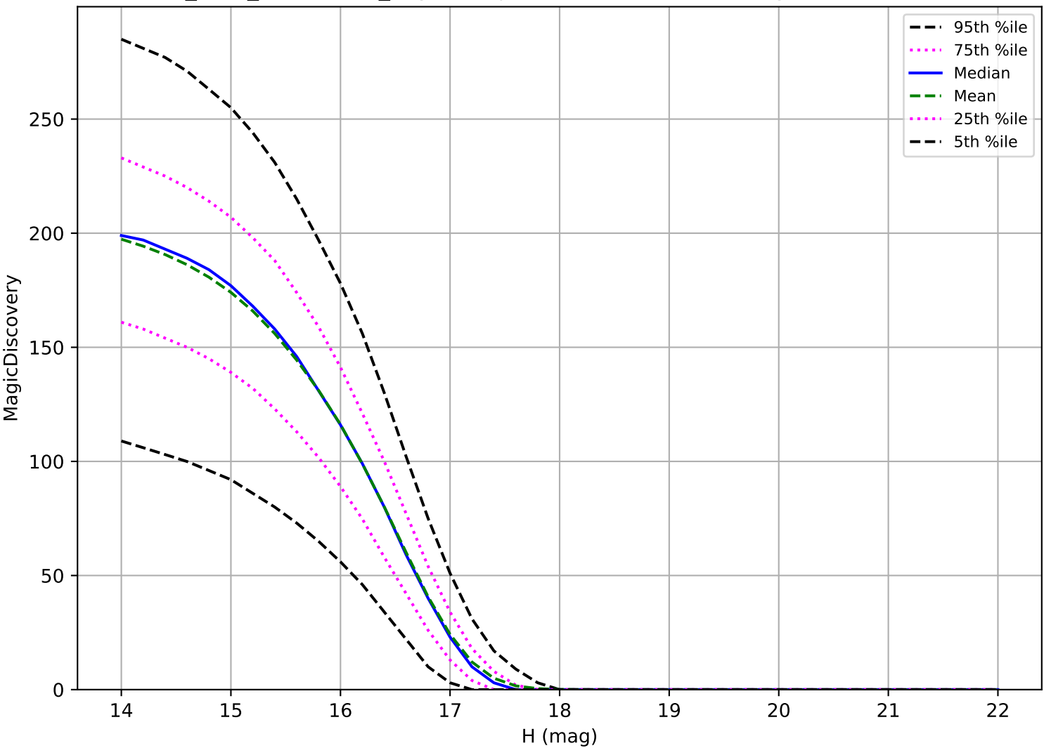
start_date_do360v3.4_10yrs: Trojan 6 detections in 60 nights detection loss
