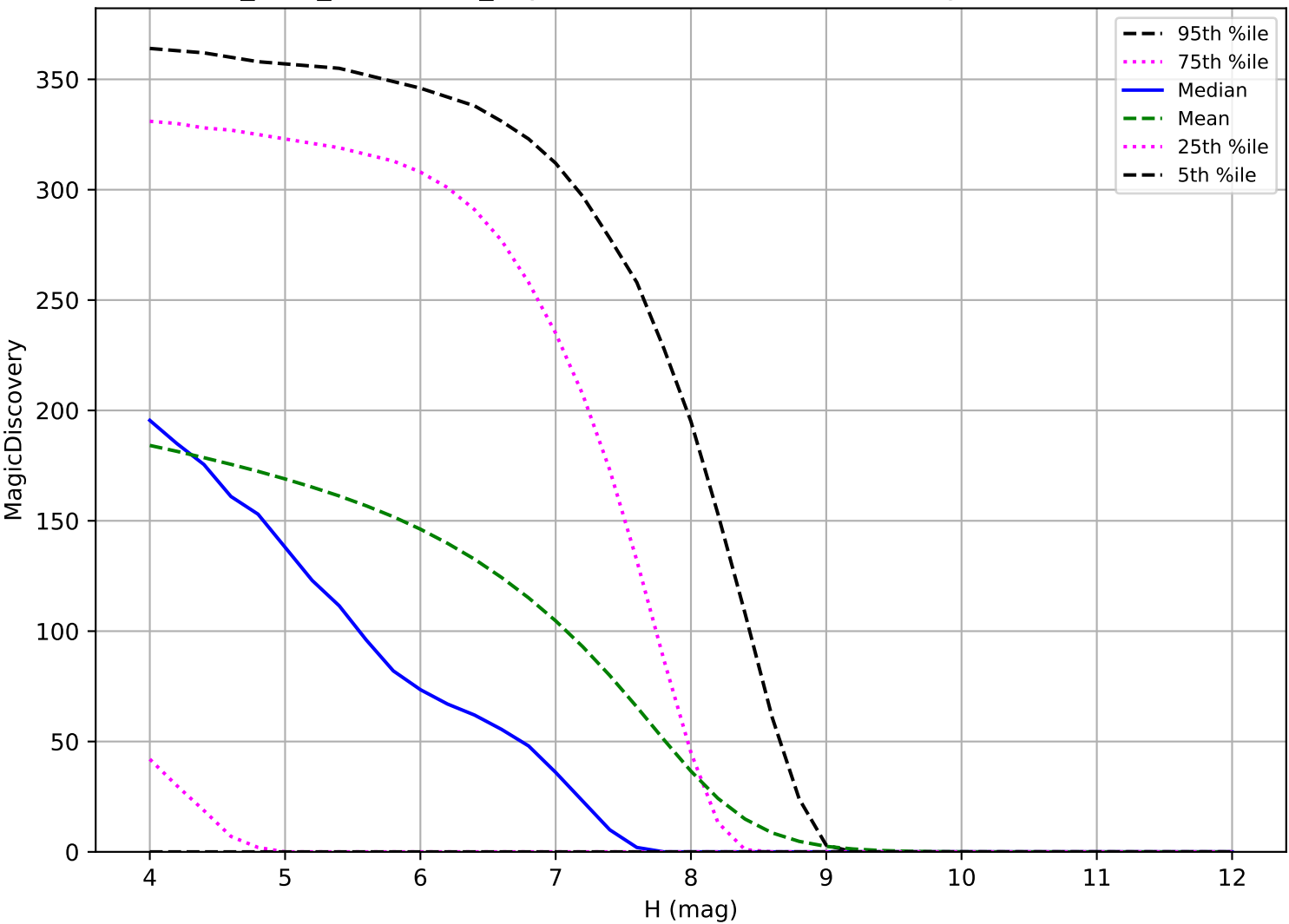
start_date_do360v3.4_10yrs: TNO 6 detections in 60 nights detection loss
