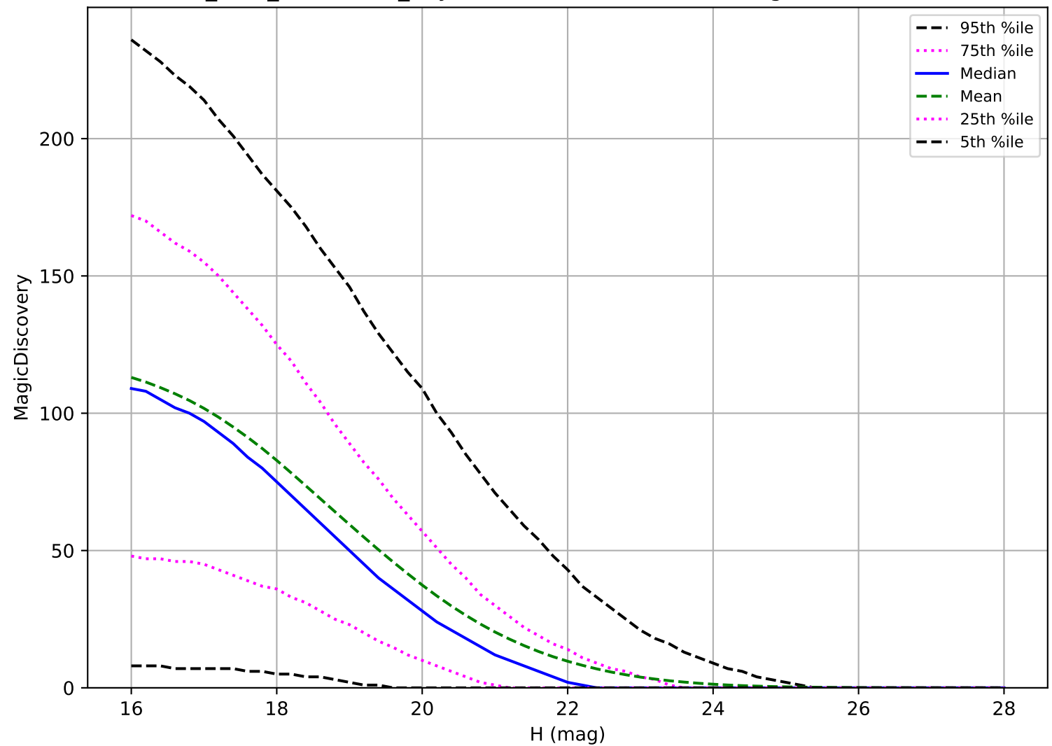
start_date_do360v3.4_10yrs: PHA 6 detections in 60 nights detection loss
