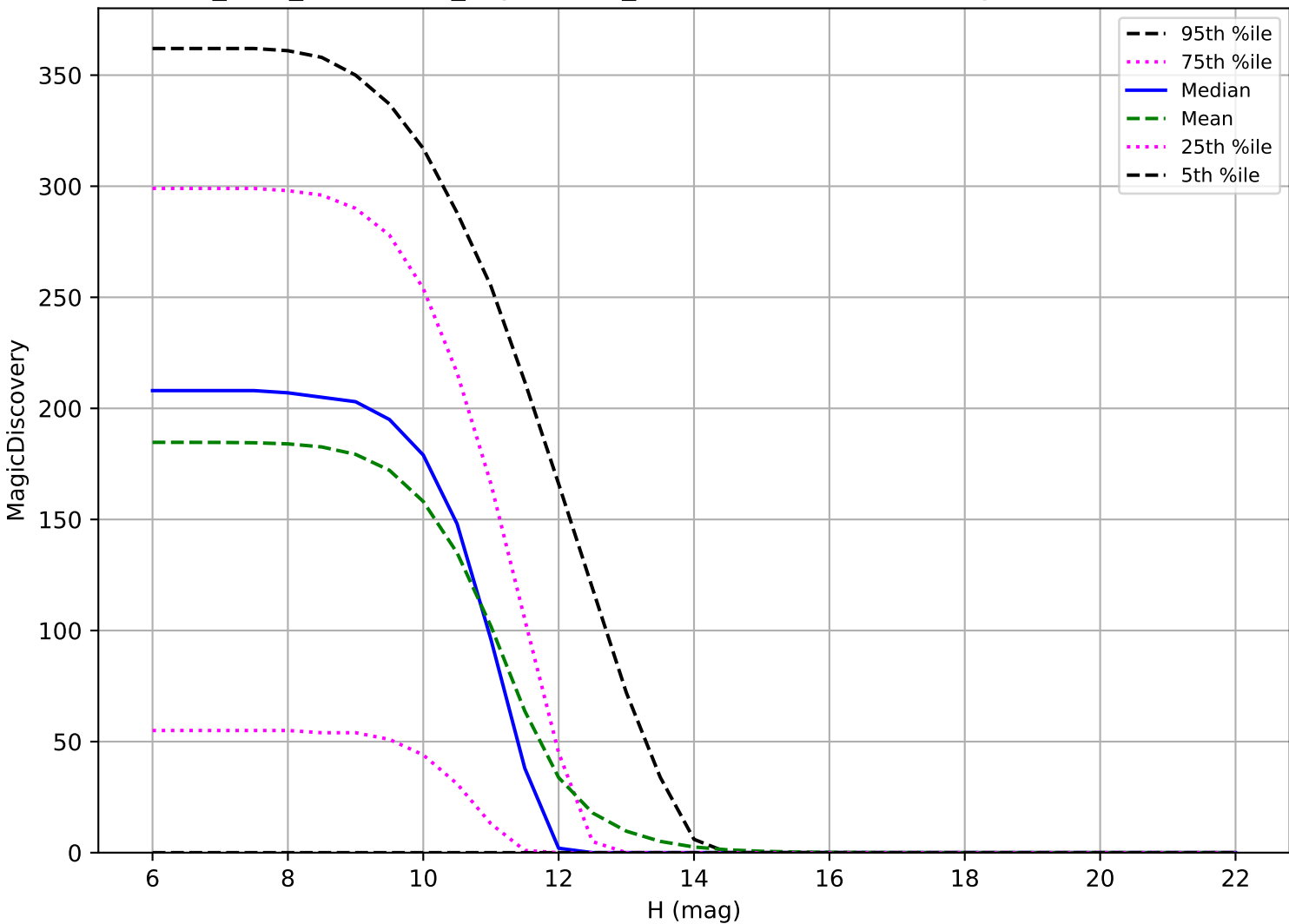
start_date_do360v3.4_10yrs: OCC_r20 6 detections in 60 nights detection loss
