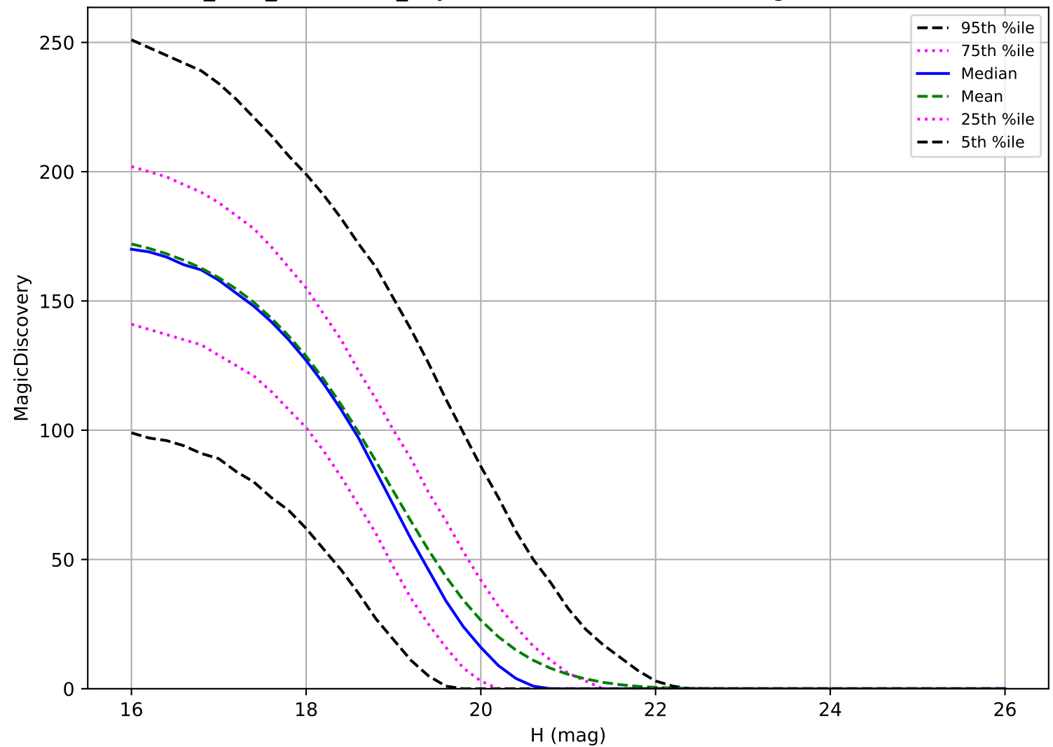
start_date_do360v3.4_10yrs: MBA 6 detections in 60 nights detection loss
